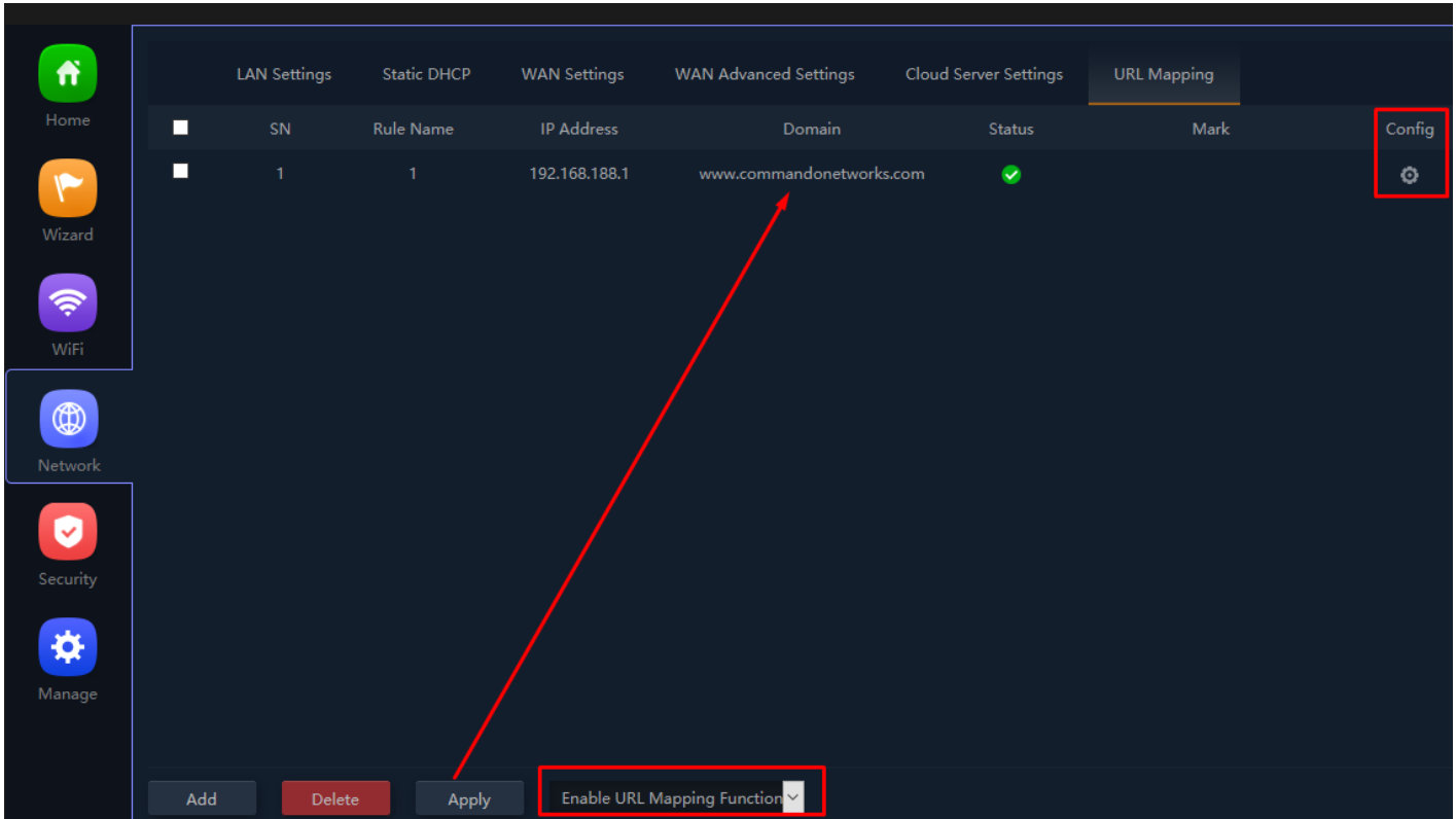
Fig 4.7.3 URL Mapping setting for AirONE AP1200
