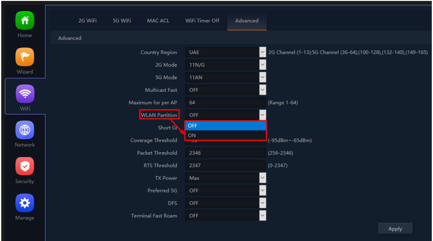
Fig 3.5.7 Selecting WLAN Partition for AirONE AP1200
