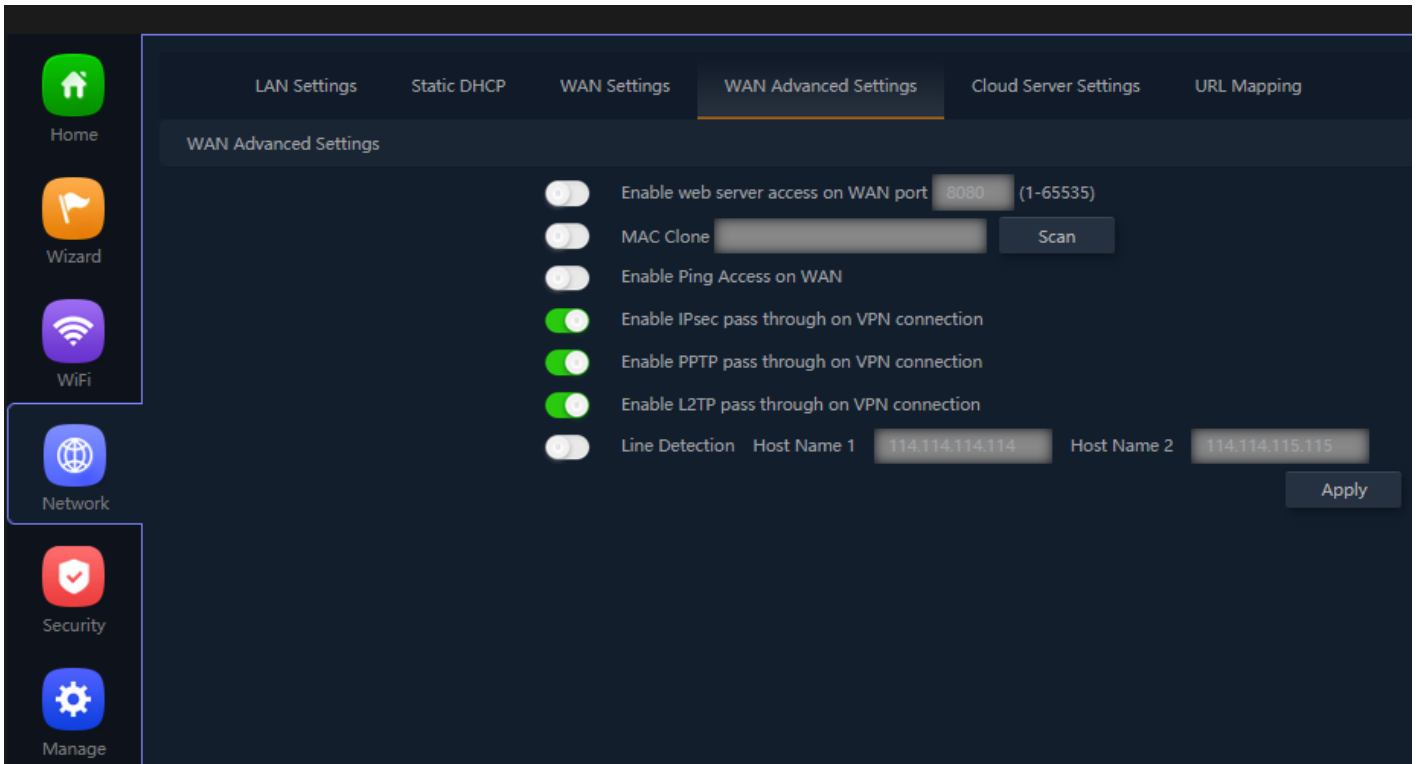
Fig 4.5.1 Default WAN Advanced Setting for AirONE AP1200
