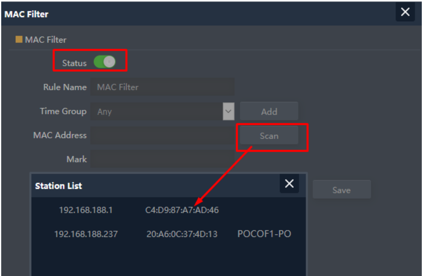
Fig 5.3.2 Setting MAC filter for AirONE AP1200
