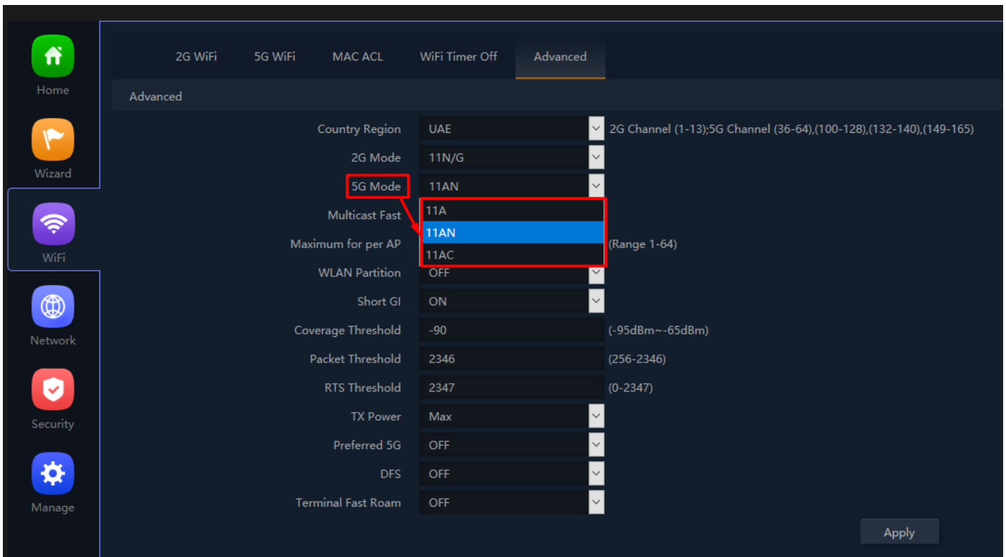
Fig 3.5.4 Selecting 5G Mode for AirONE AP1200
