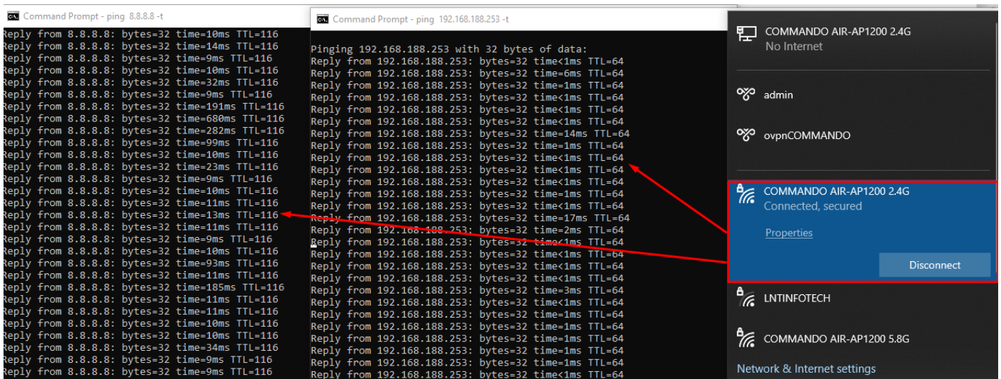
Fig 2.3.9 WISP mode Ping response of Client of AirONE AP1200
