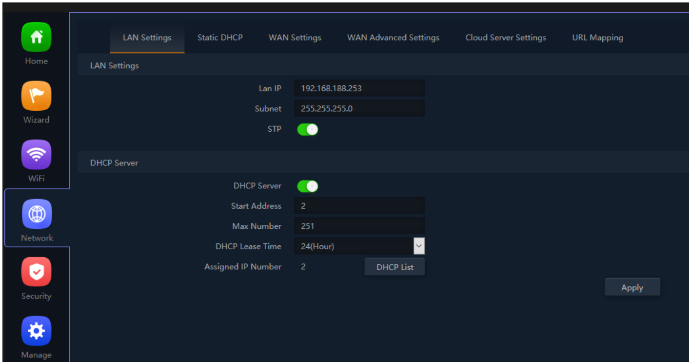
Fig 4.1.1 Setting LAN IP which used as access IP for AirONE AP1200
