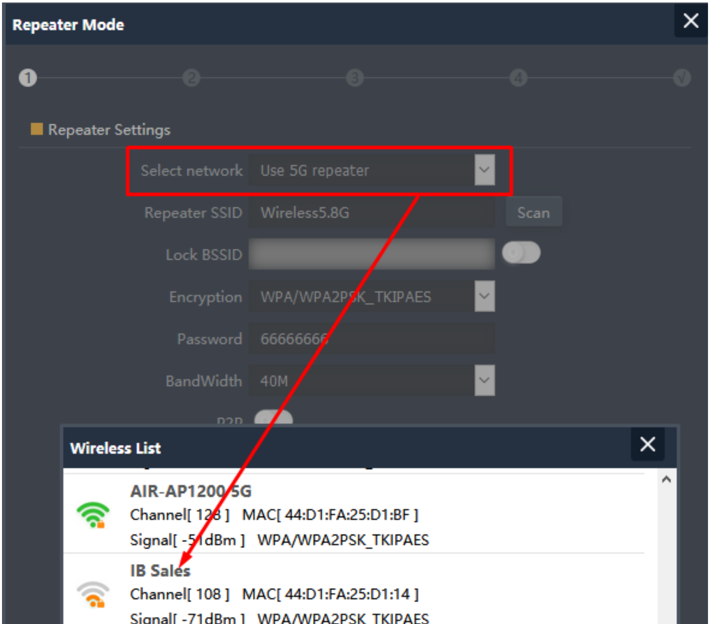
Fig 2.3.3 Selecting 5G Repeater SSID of AirONE AP1200
