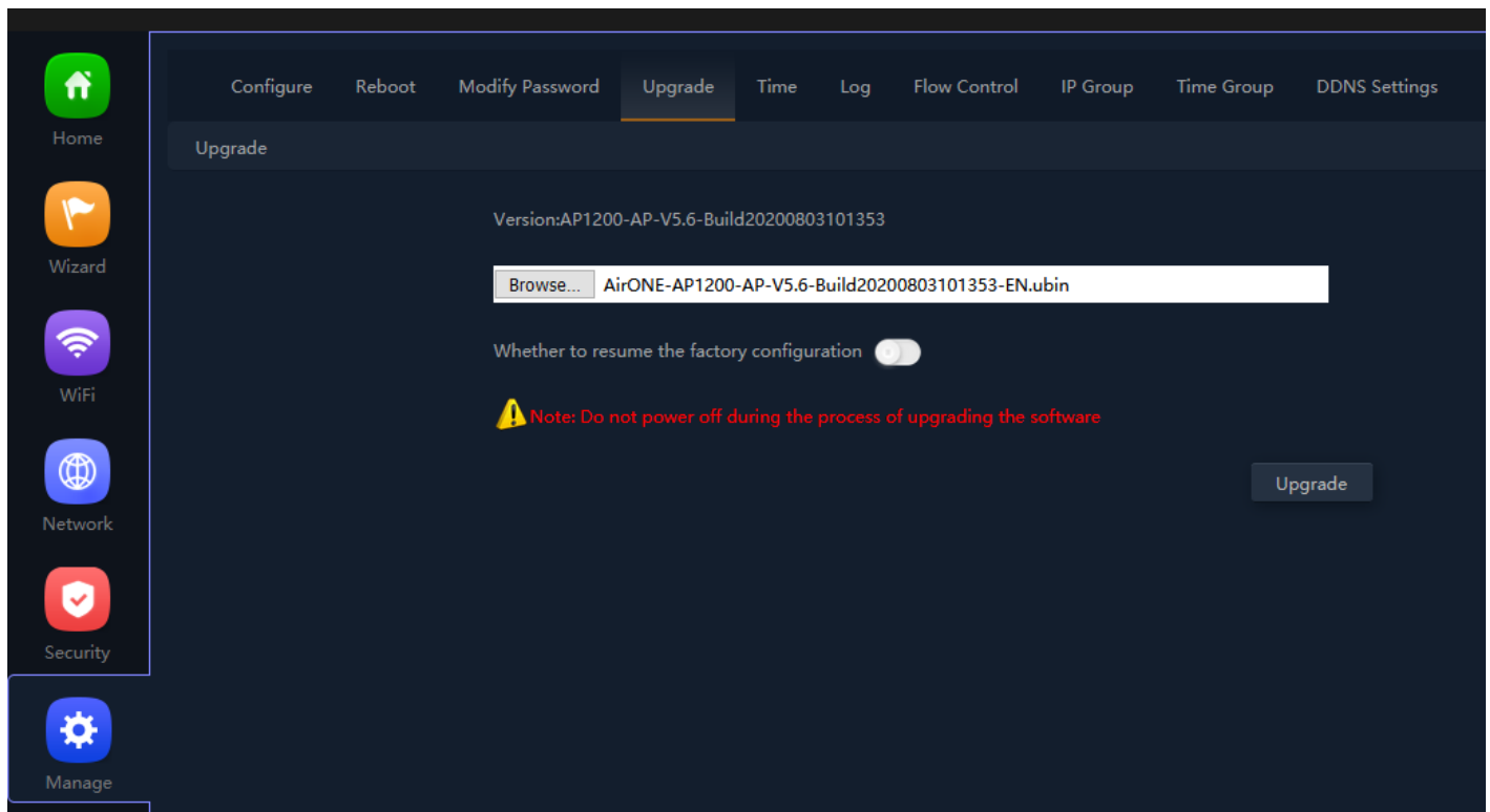
Fig 6.4.1 Default Upgrade page for AirONE AP1200
