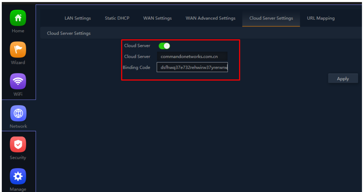
Fig 4.6.2 Enabling Cloud server setting for AirONE AP1200
