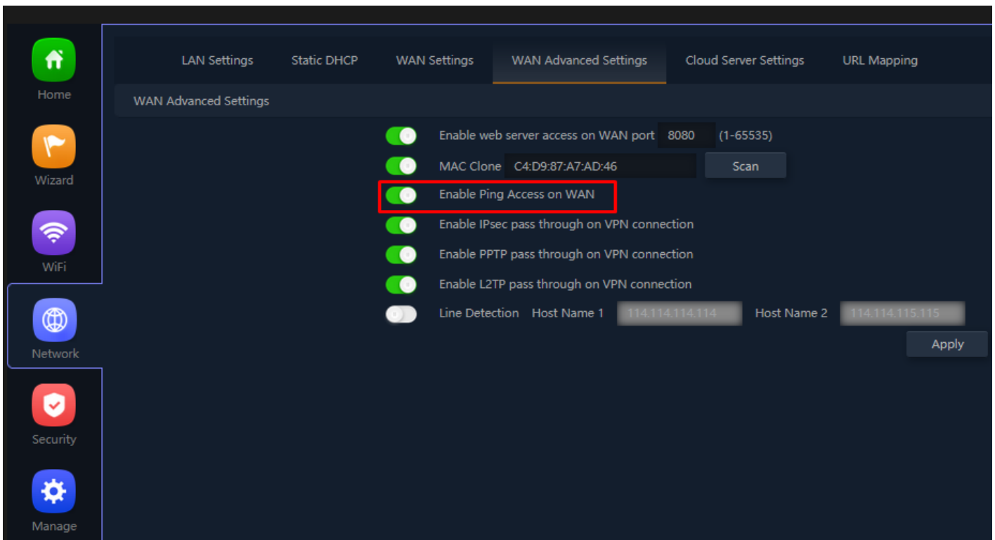
Fig 4.5.4 Enabling Ping access through WAN for AirONE AP1200
