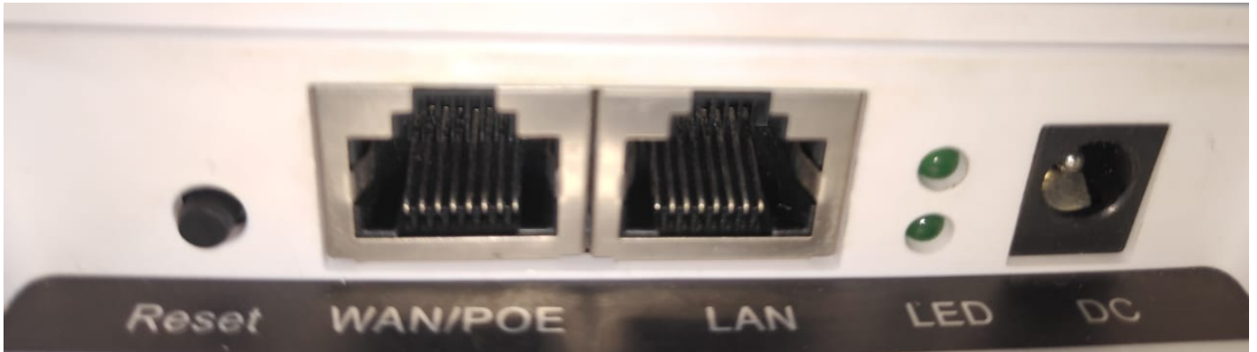
Fig 1. Physical port on AirONE AP1200
