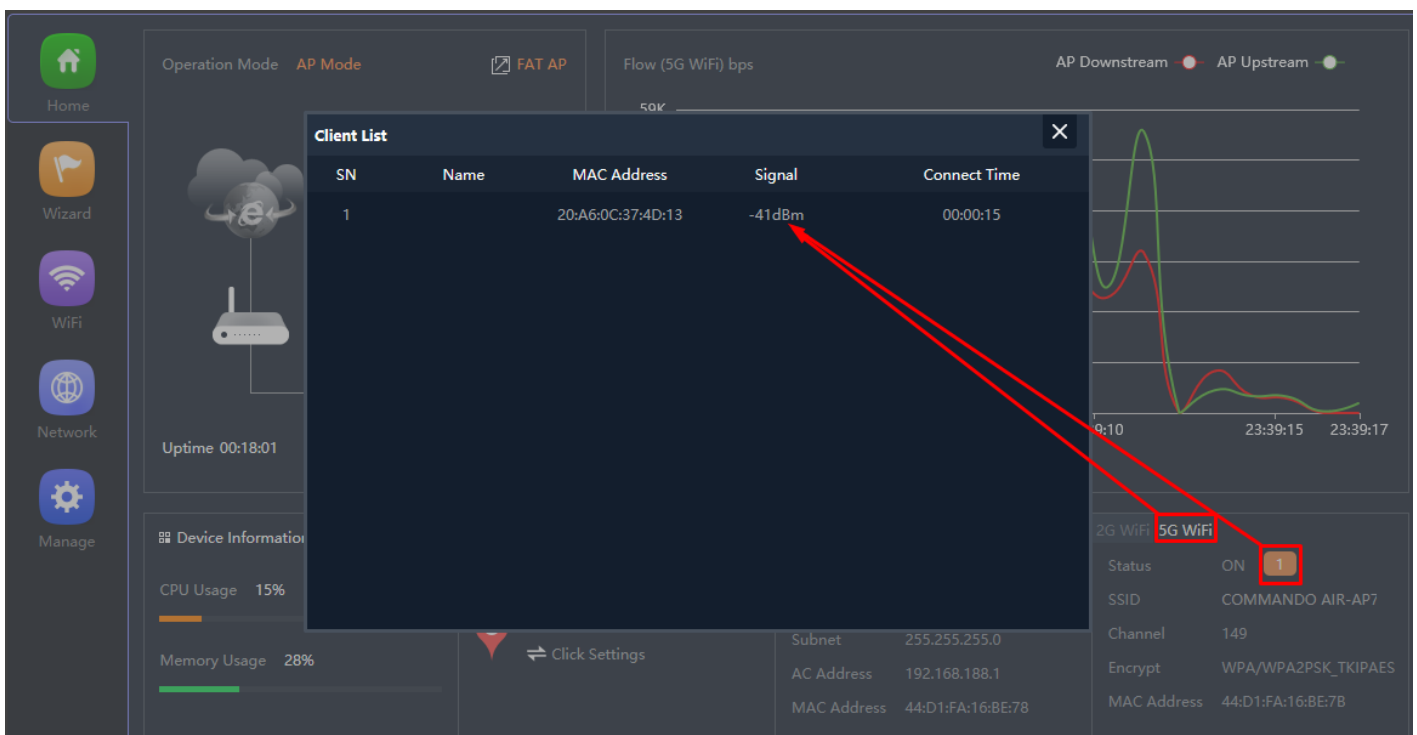
Fig 1.4.2 Clients list of 5G Wi-Fi AirONE AP1200
