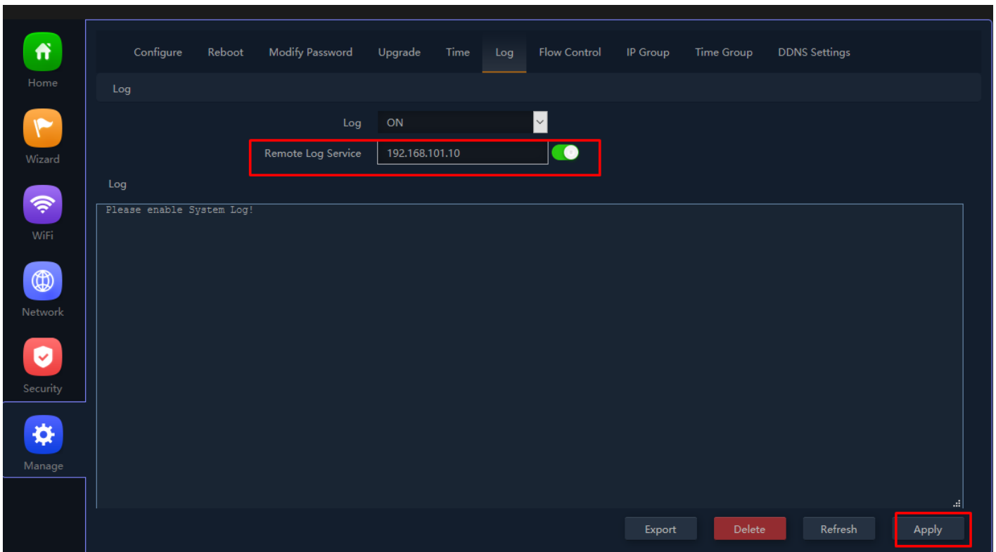
Fig 6.6.3 Remote Log service setting IP for AirONE AP1200
