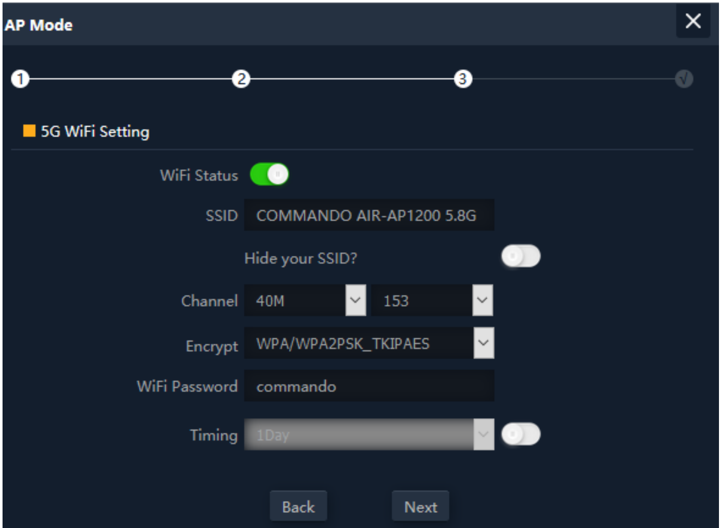
Fig 2.4.4 Setting 5G Wi-Fi for AP mode of AirONE AP1200
