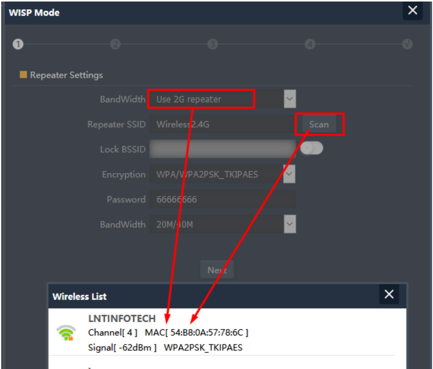
Fig 2.3.2 2G Repeater Setting WISP mode of AirONE AP1200
