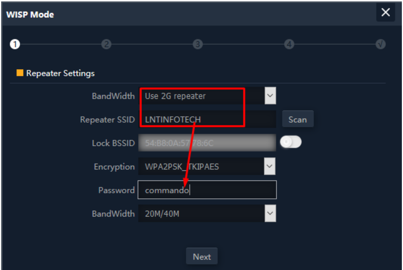
Fig 2.3.4 Repeater SSID for 2G repeater WISP mode of AirONE AP1200
