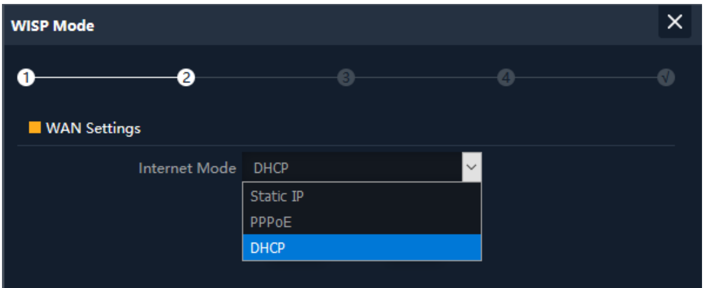
Fig 2.3.5 WAN Setting WISP mode of AirONE AP1200
