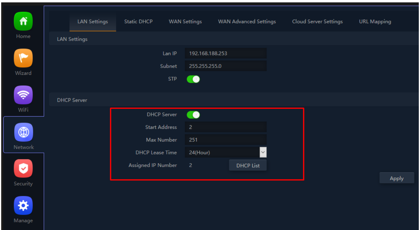
Fig 4.1.3 Setting DHCP for AirONE AP1200
