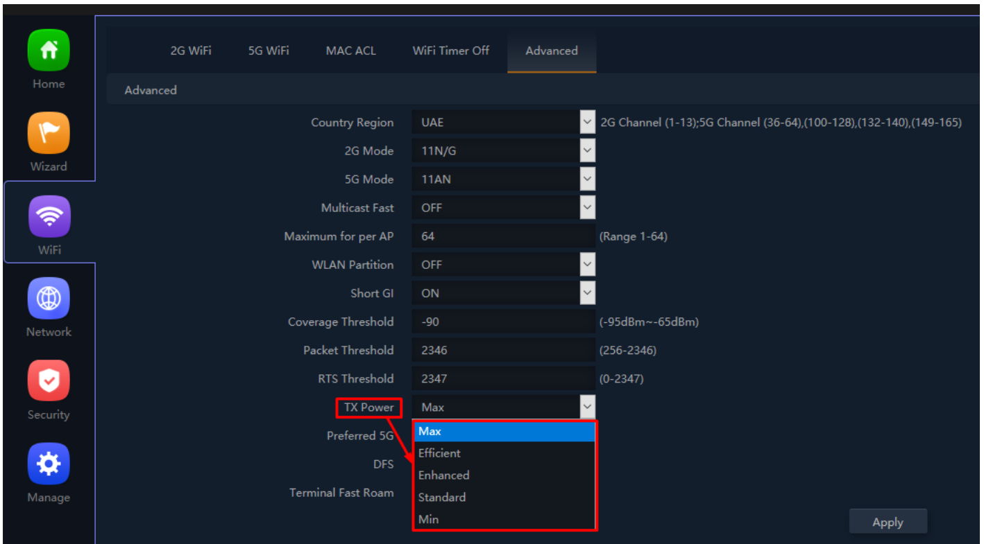
Fig 3.5.10 Setting Tx Power for AirONE AP1200
