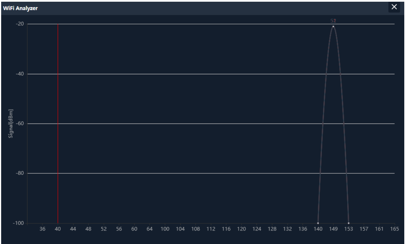
Fig 3.1.6 5G Wi-Fi Analyzer of AirONE AP1200
