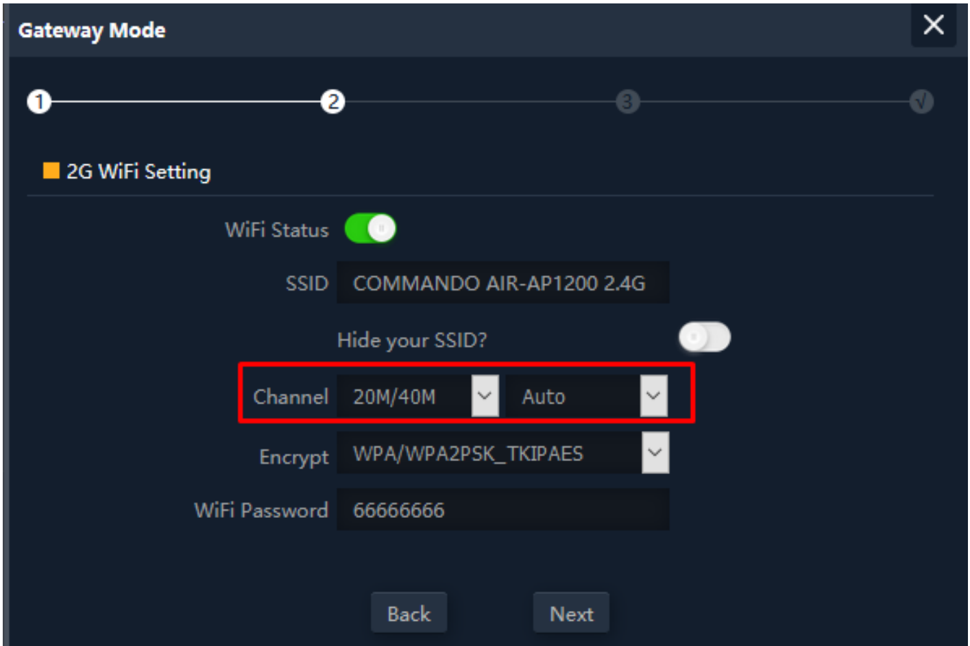
Fig 2.1.3 Gateway mode 2G Wi-Fi Setting of AirONE AP1200
