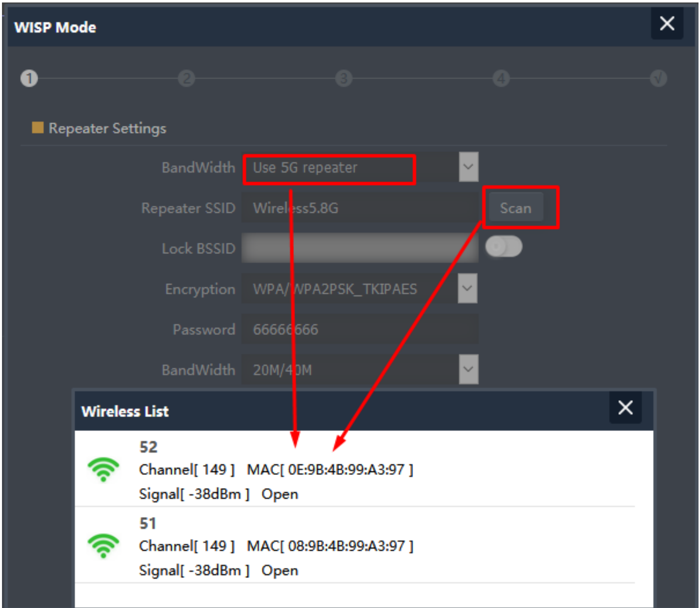
Fig 2.3.3 5G Repeater Setting WISP mode of AirONE AP1200
