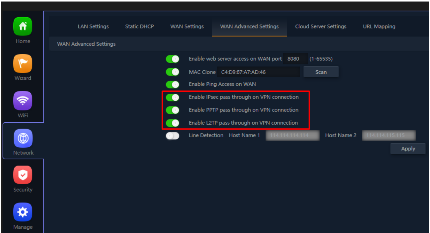
Fig 4.5.5 Enabling IPsec/PPTP/L2TP access through VPN for AirONE AP1200
