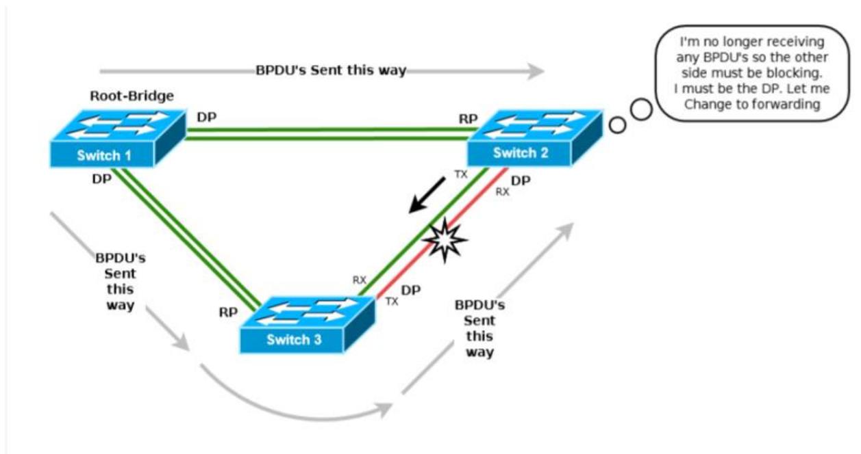
Fig 34.2 BPDU Route
