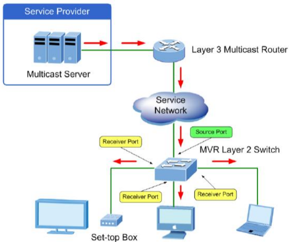
Fig 20.1 MVR concept
