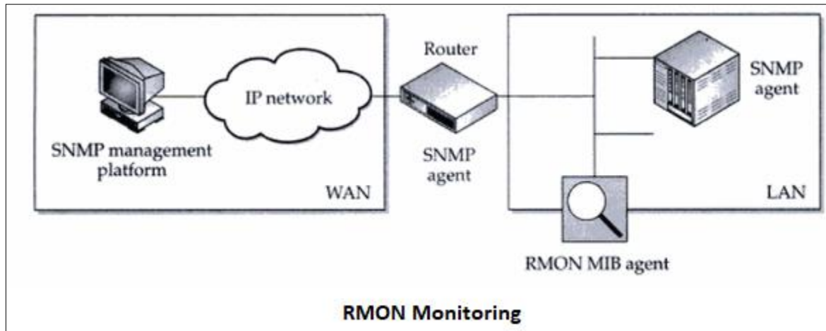
Fig 27.1 RMON Monitoring
